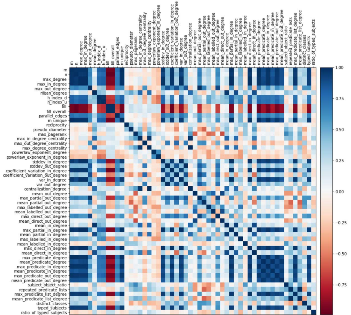
Fig. 1. Correlation matrix. Shows the whole set of measures and their color-encoded Spearman correlation coefficient. Values close to 1.0 indicate strong positive correlation, around 0 no correlation, and close to -1.0 strong negative correlation.
