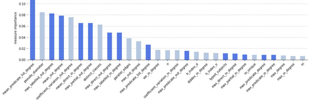
Fig. 6. Overall measure importance while discriminating datasets (classification task (1)). Shown are mean values for all non-redundant measures m \in M' . Colors encode graph measures (in light) and RDF graph measures.
