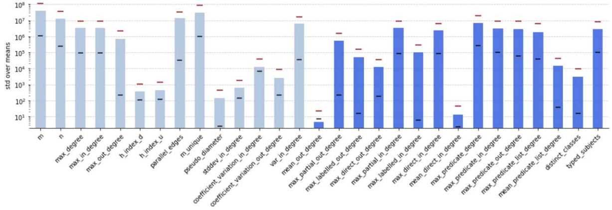
Fig. 5. Degree of variance across knowledge domains. A low/high value indicates low/high variance across knowledge domains. Colors encode graph measures (in light) and RDF graph measures. y-axis is log-scaled.
